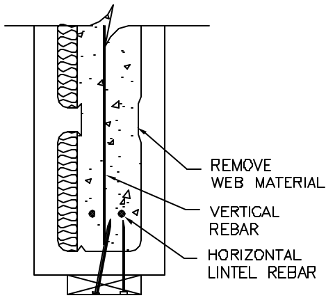
LINTEL FORM (SITE-ALTERED END UNIT)
