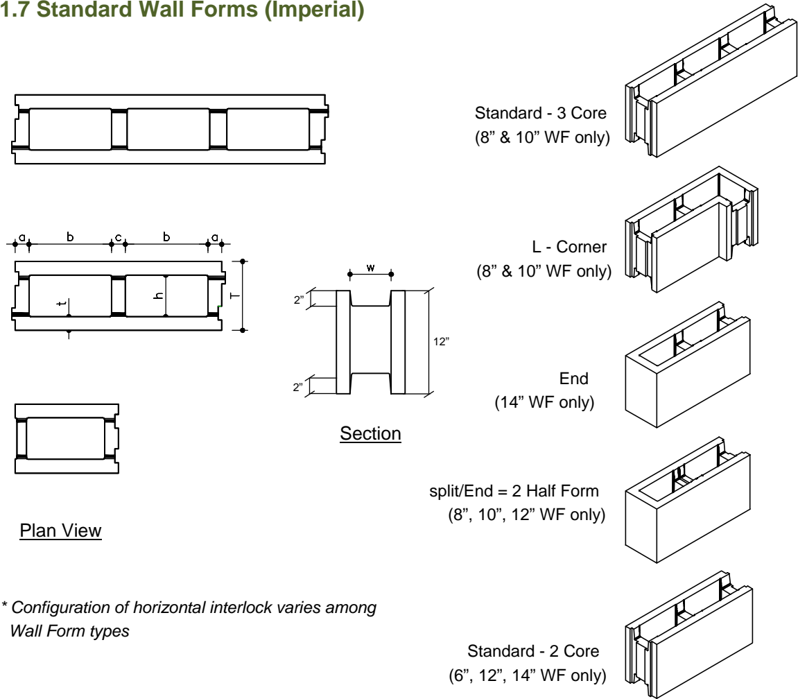
Figure 1.2 - Standard Wall Form Schematic
