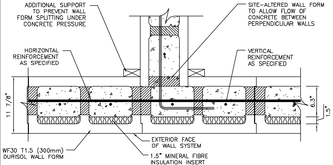
T-WALL CONFIGURATION (ALTERNATE COURSE)
