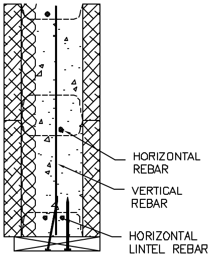
STANDARD COURSE LINTEL
