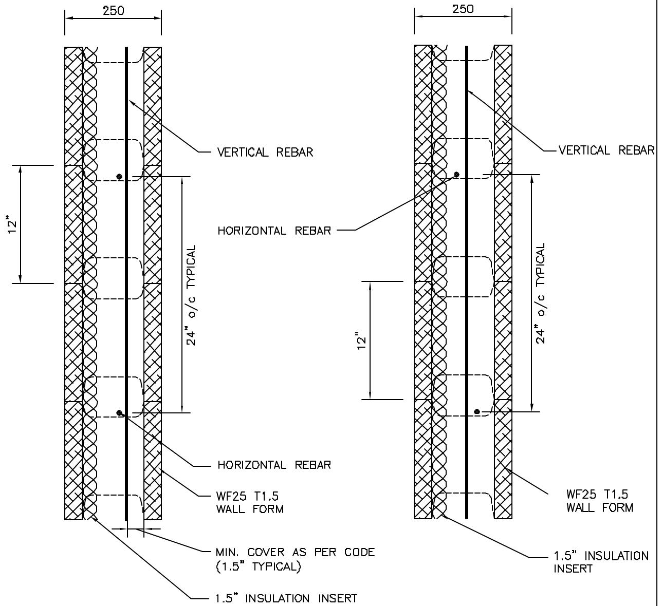
VERTICAL BARS OFF-CENTER (TYPICAL BELOW-GRADE)
