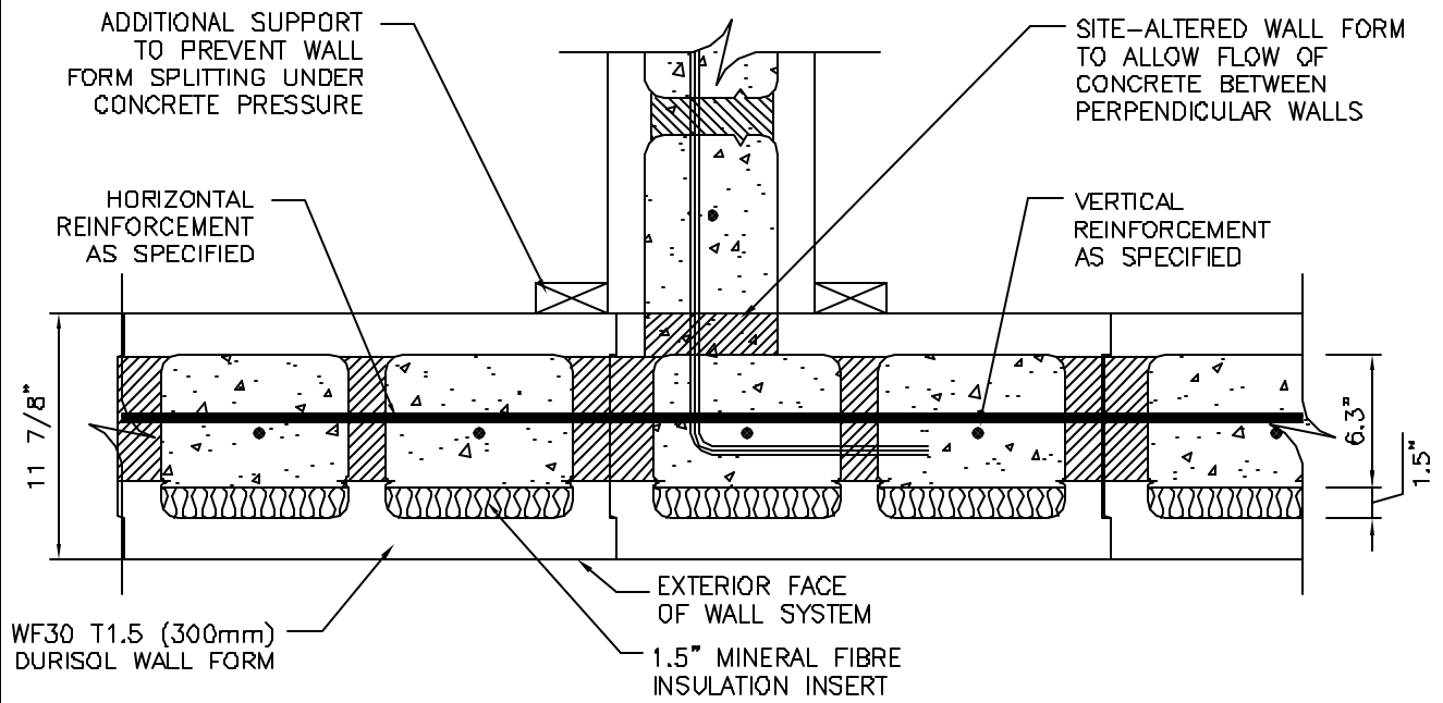
T-WALL CONFIGURATION (FIRST COURSE)
